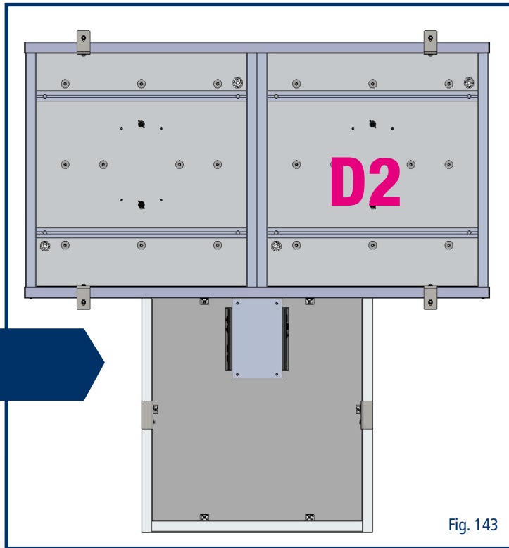
Rear view of the twall® D2
