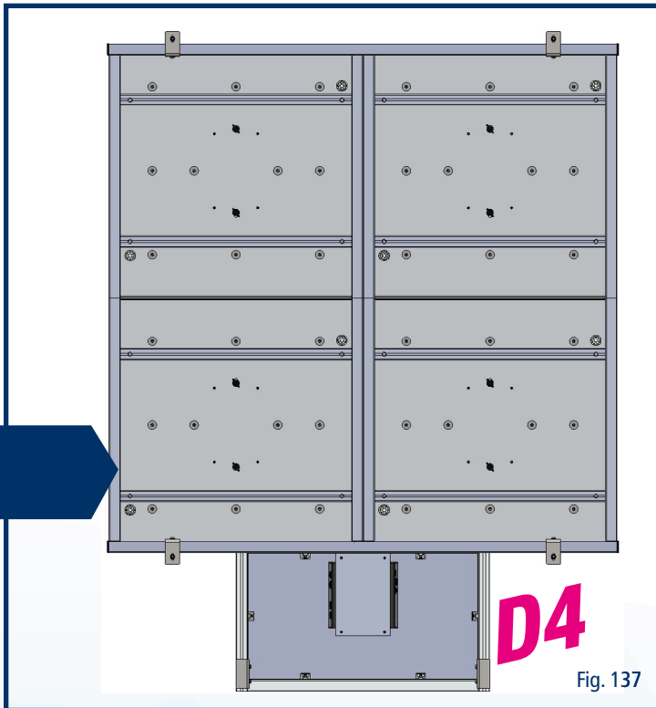
Rear view of the twall® D4
